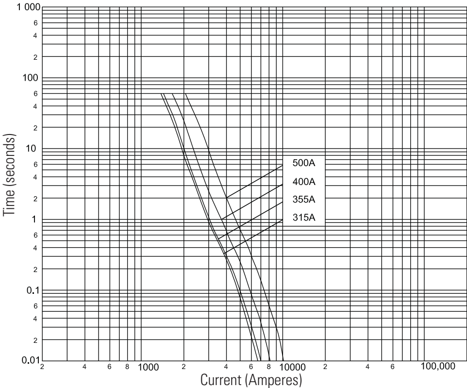
NH Size 3 - Time current curve
